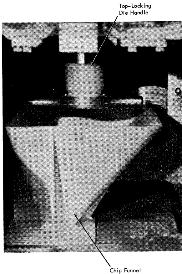
Figure 8. Punch Die (Top-Locking)
