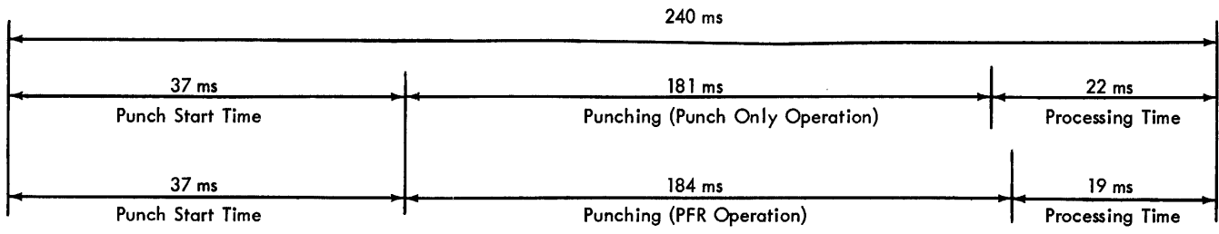
Figure 13. Punch Timing
